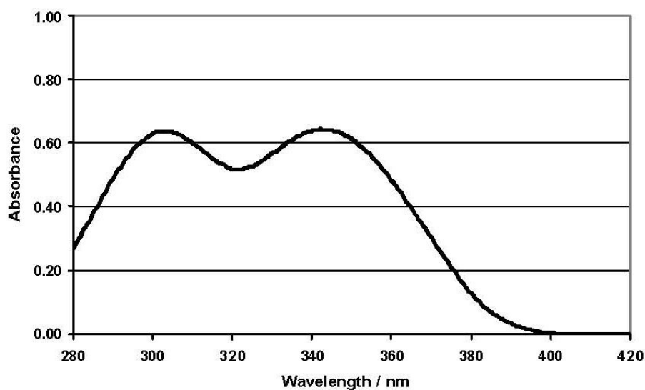
UV Absorbance Spectrum (40 mg/l in chloroform, cell thickness = 1 cm)
