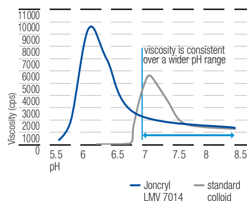
Figure 3: Viscosity vs. pH (22% solids)
